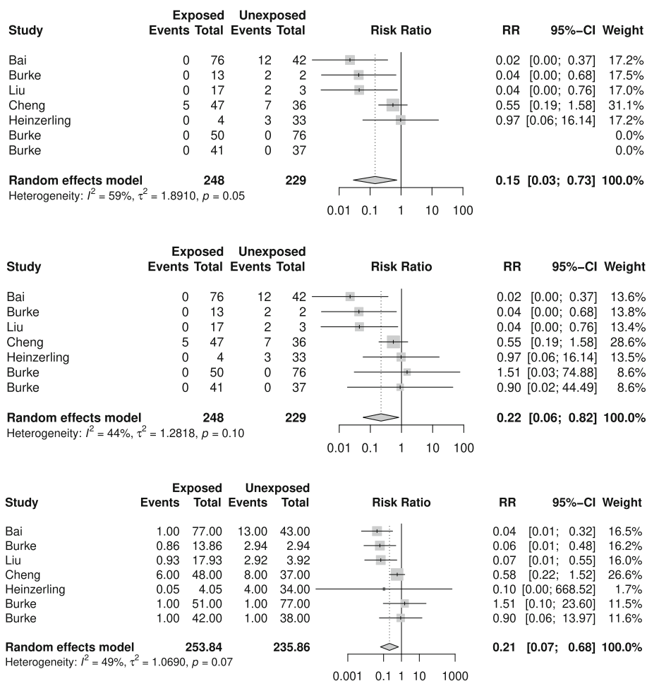
FIGURE 6. Forest plots on the relative risk between physical distancing and infection for COVID-19 data.
