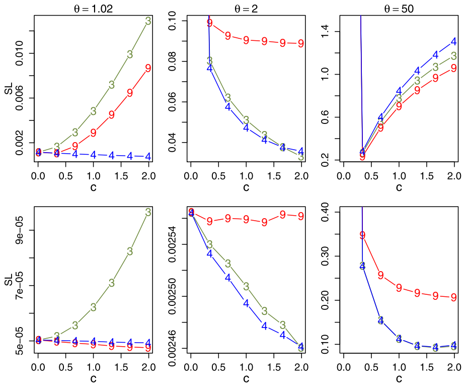
FIGURE 1. The Stein losses for the shrinkage estimators from the three families with \theta = 1.02, 2 or 50, n = 10 (top three panels) or 200 (bottom three panels), and c \in (0, 2) , where ‘3’ represents the estimators from family (3), ‘4’ represents the estimators from family (4), and ‘9’ represents the estimators from family (9).
