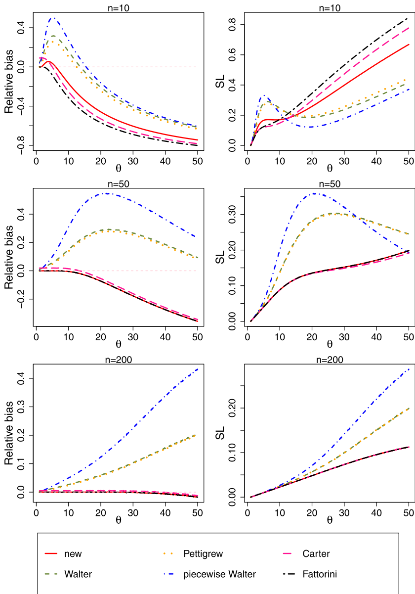
FIGURE 5. The relative biases and the Stein losses of the six estimators with n = 10, 50 or 200 .
